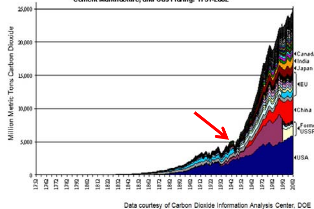
Figure 2: Global CO 2 Emissions from Fossil Fuel Burning, Cement Manufacture, and Gas Flaring: 1751-2002
